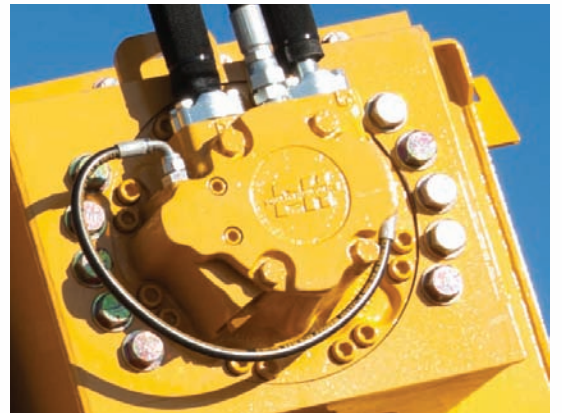
Loop-flush return system provides thermal relief
